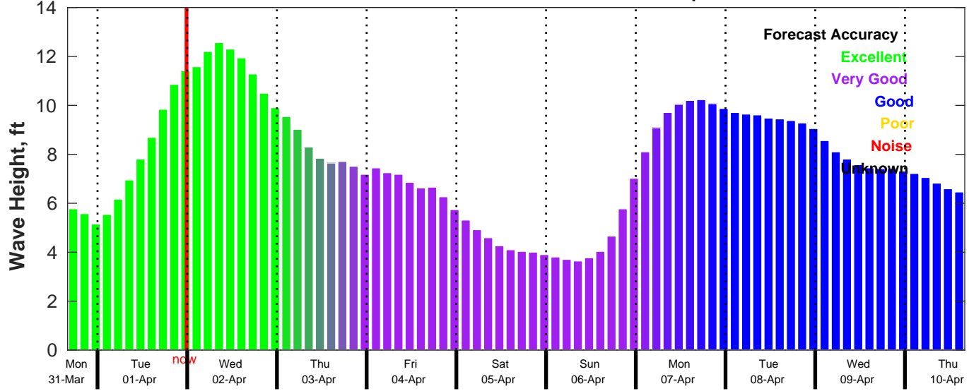
CMEMS Wave Forecast for NDBC 46054 from 31-Mar-2025 16:00:00 to 10-Apr-2025 16:00:00
