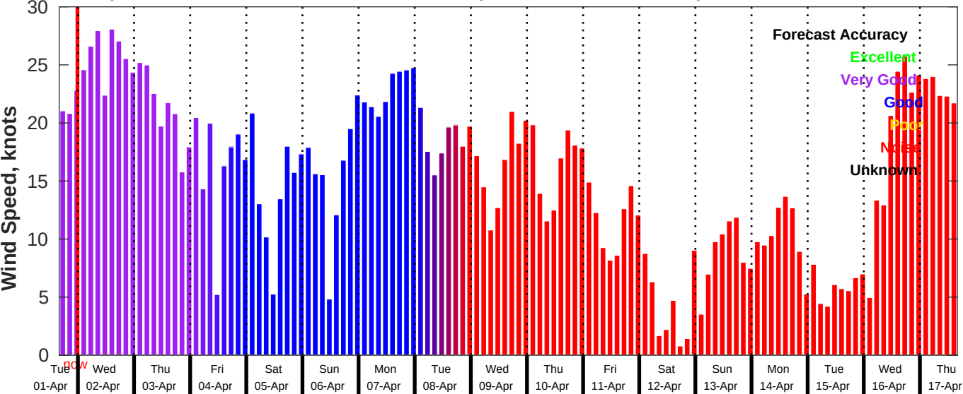
GFS Wind Speed Forecast for NDBC 46054 from 01-Apr-2025 16:00:00 to 17-Apr-2025 16:00:00
