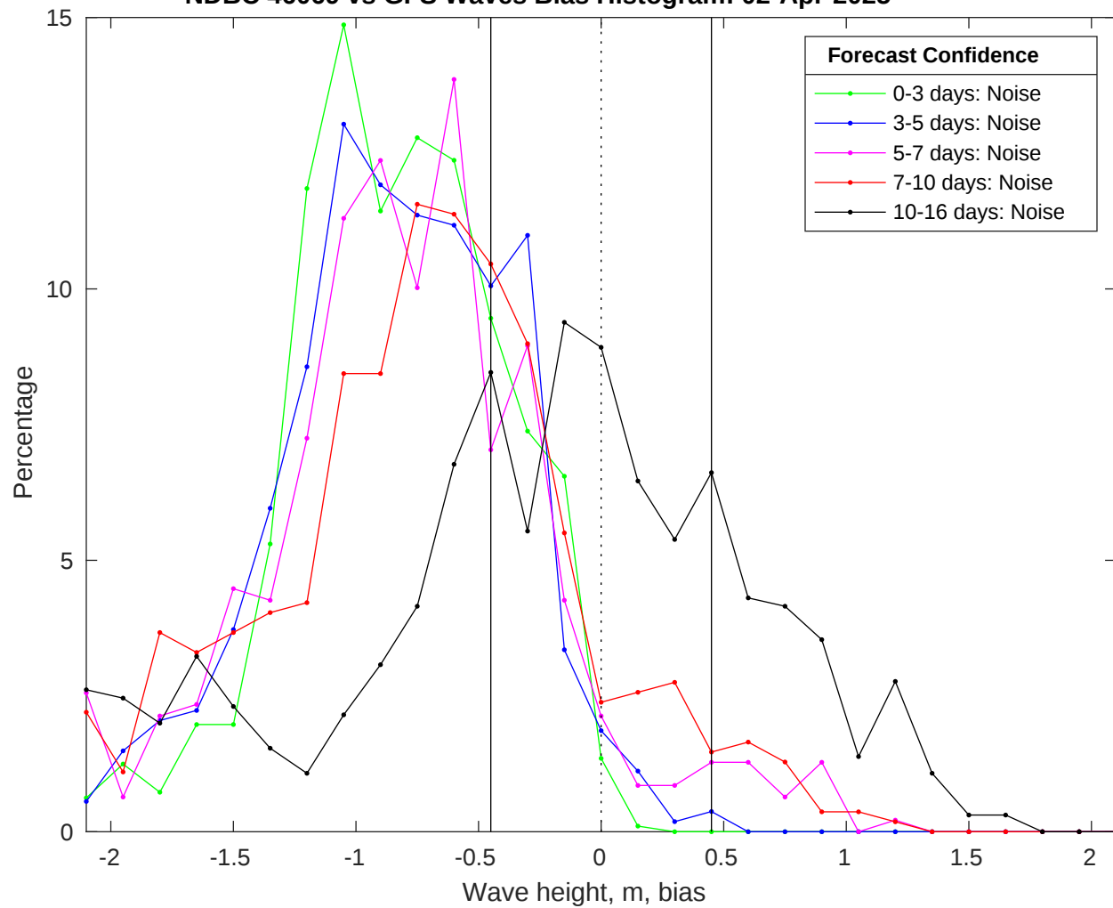
NDBC 46069 vs GFS Waves Bias Histogram: 02-Apr-2025
