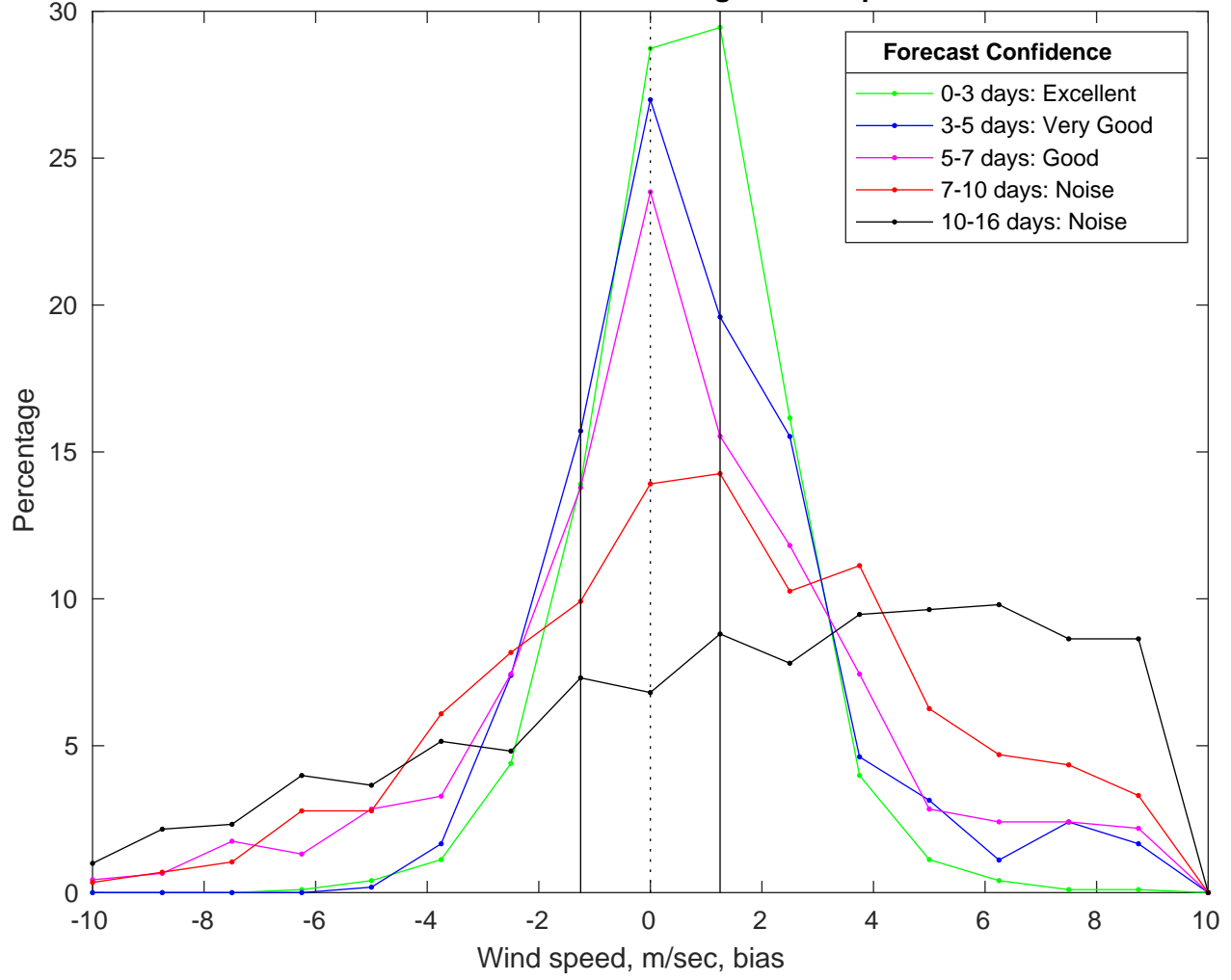
NDBC 46069 vs GFS Winds Bias Histogram: 02-Apr-2025
