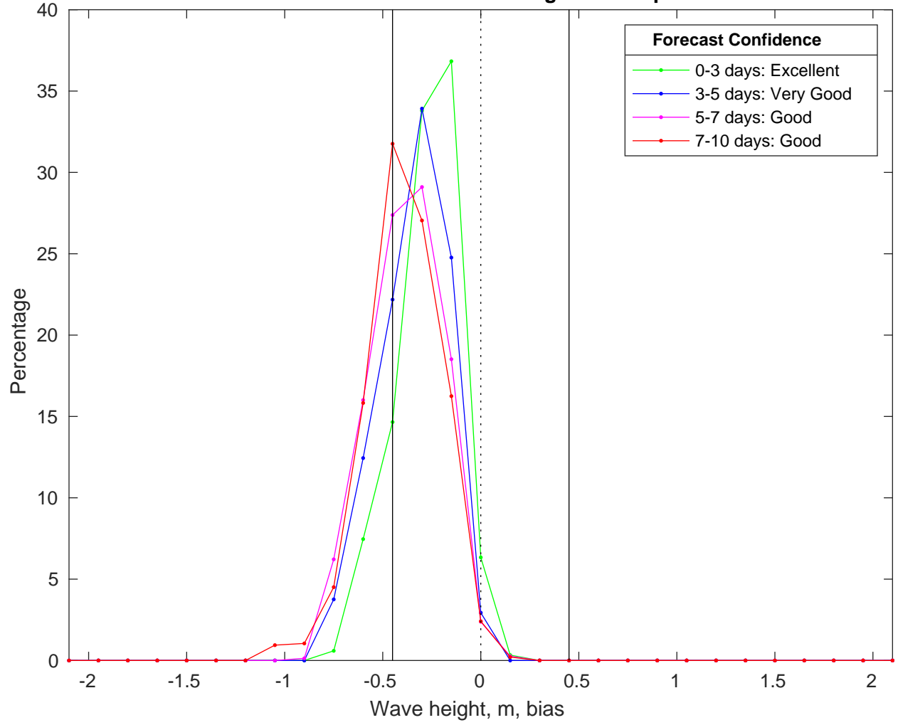
NDBC 51209 vs CMEMS Waves Bias Histogram: 02-Apr-2025
