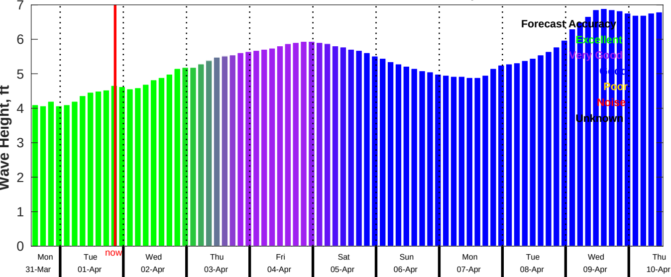
CMEMS Wave Forecast for NDBC 51209 from 31-Mar-2025 13:00:00 to 10-Apr-2025 13:00:00
