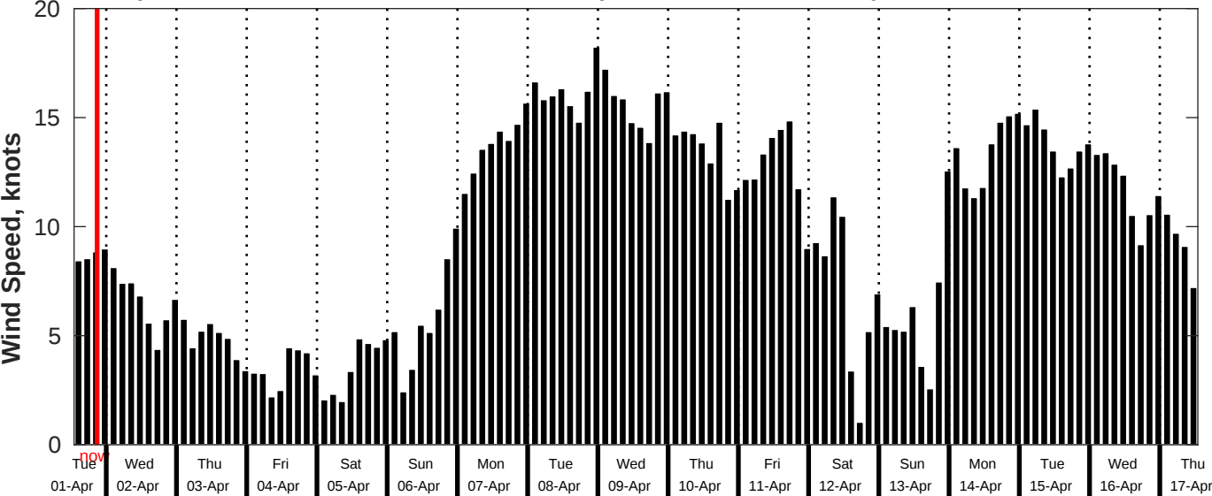
GFS Wind Speed Forecast for NDBC 51209 from 01-Apr-2025 13:00:00 to 17-Apr-2025 13:00:00
