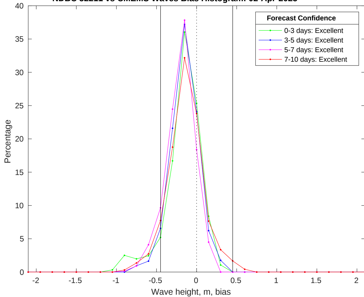
NDBC 52211 vs CMEMS Waves Bias Histogram: 02-Apr-2025
