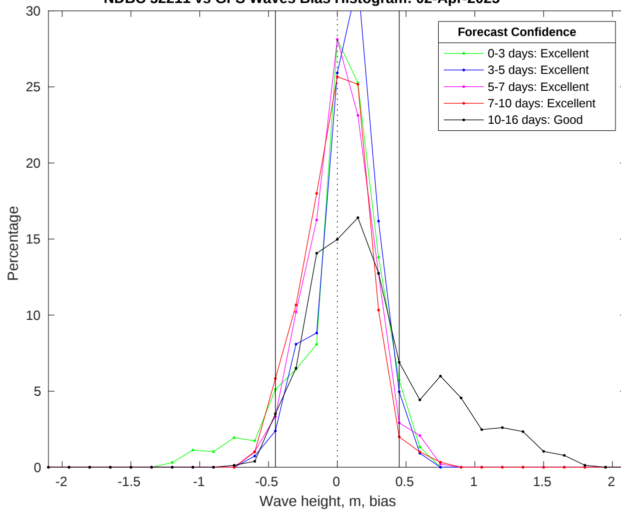
NDBC 52211 vs GFS Waves Bias Histogram: 02-Apr-2025
