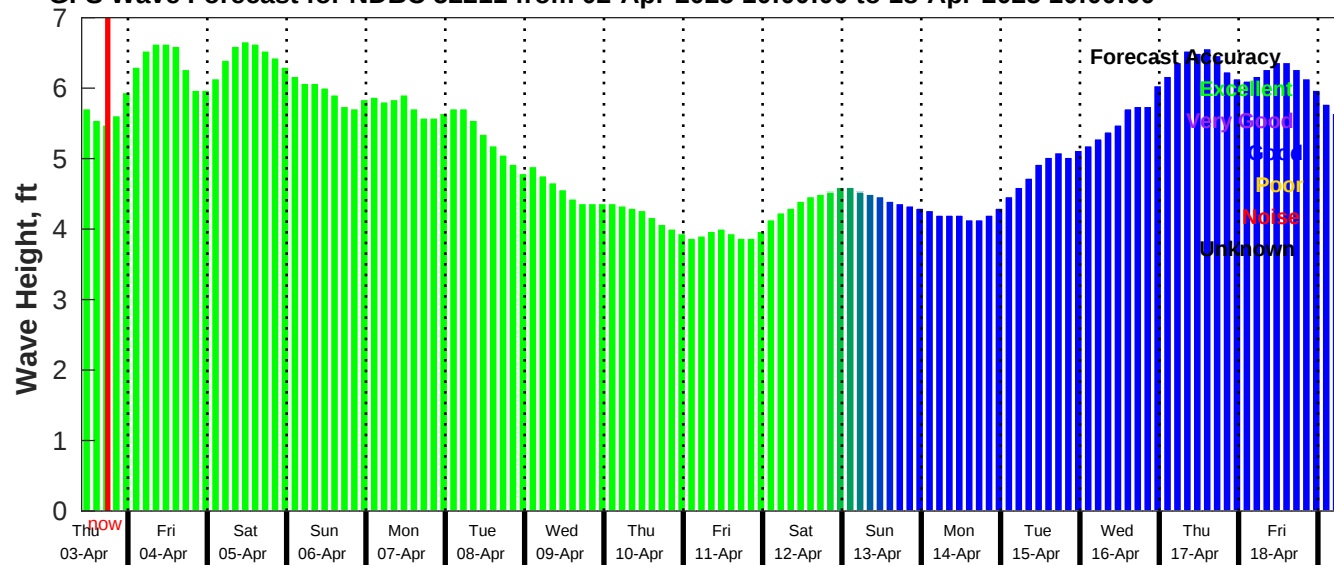
GFS Wave Forecast for NDBC 52211 from 02-Apr-2025 10:00:00 to 18-Apr-2025 10:00:00
