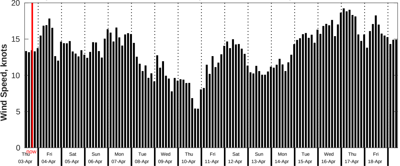
GFS Wind Speed Forecast for NDBC 52211 from 02-Apr-2025 10:00:00 to 18-Apr-2025 10:00:00
