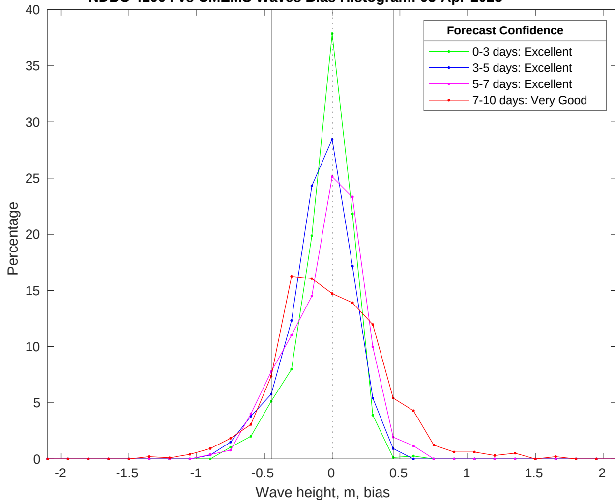
NDBC 41004 vs CMEMS Waves Bias Histogram: 03-Apr-2025
