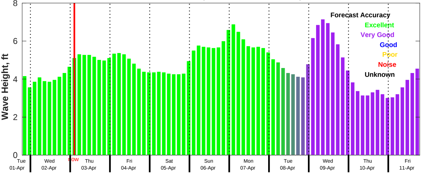
CMEMS Wave Forecast for NDBC 41004 from 01-Apr-2025 19:00:00 to 11-Apr-2025 19:00:00
