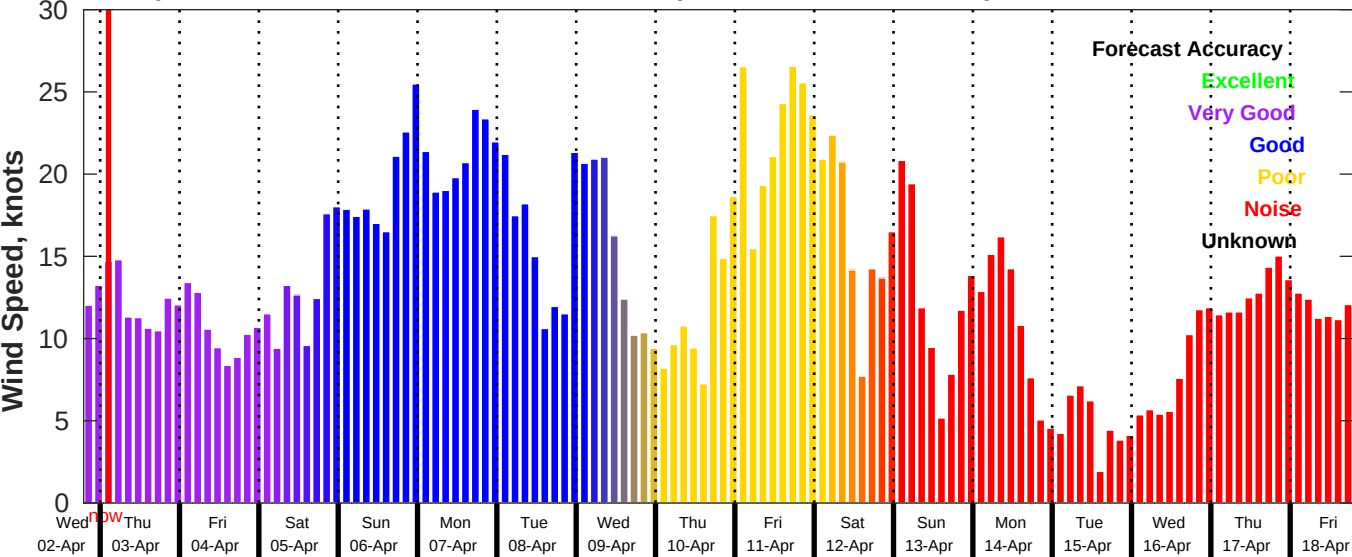
GFS Wind Speed Forecast for NDBC 41004 from 02-Apr-2025 19:00:00 to 18-Apr-2025 19:00:00
