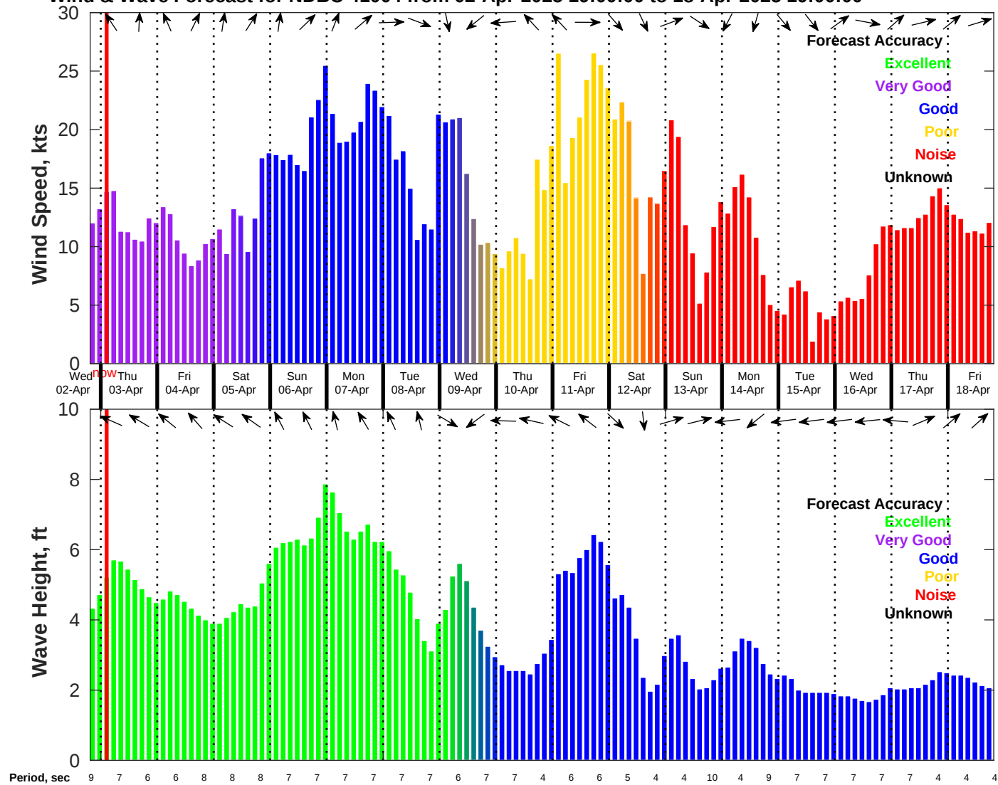
Wind & Wave Forecast for NDBC 41004 from 02-Apr-2025 19:00:00 to 18-Apr-2025 19:00:00
