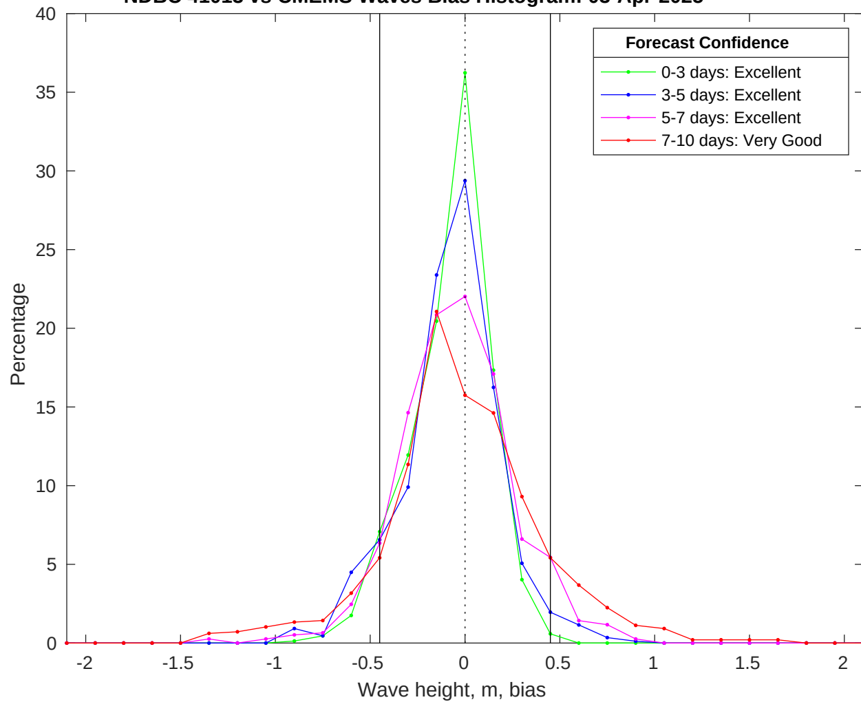
NDBC 41013 vs CMEMS Waves Bias Histogram: 03-Apr-2025
