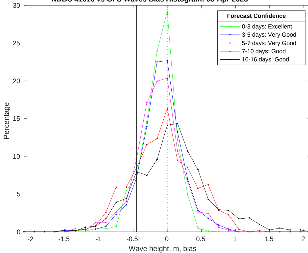
NDBC 41013 vs GFS Waves Bias Histogram: 03-Apr-2025
