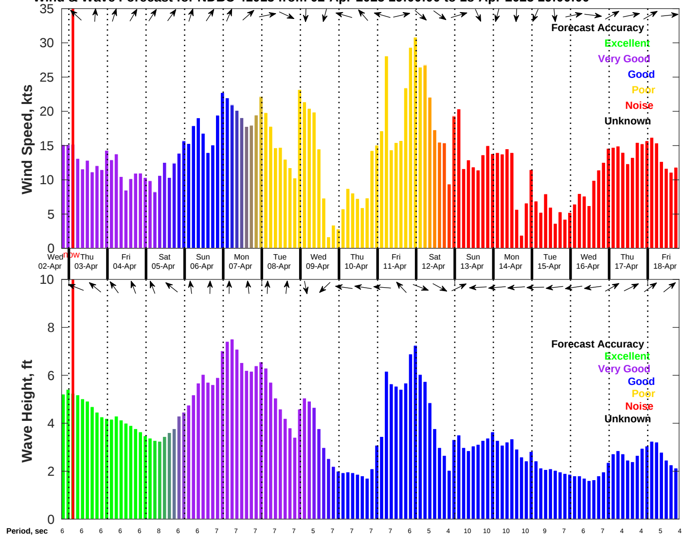
Wind & Wave Forecast for NDBC 41013 from 02-Apr-2025 19:00:00 to 18-Apr-2025 19:00:00
