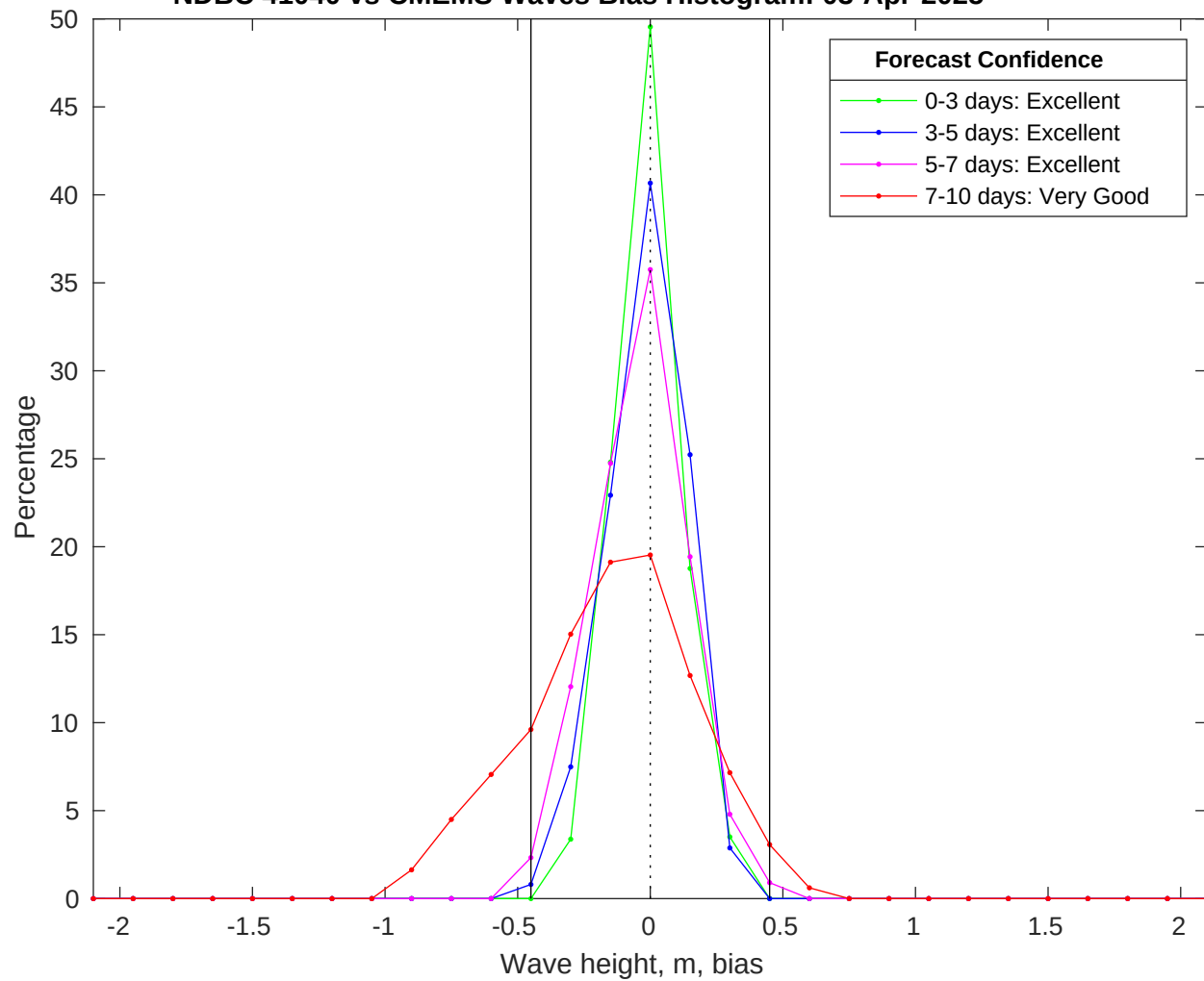
NDBC 41040 vs CMEMS Waves Bias Histogram: 03-Apr-2025
