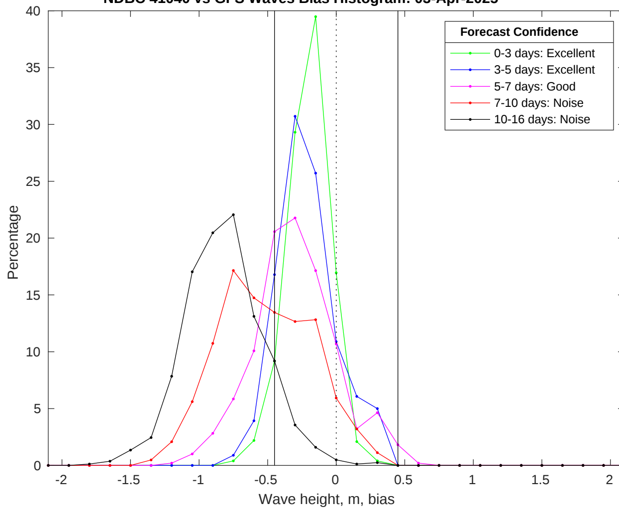
NDBC 41040 vs GFS Waves Bias Histogram: 03-Apr-2025
