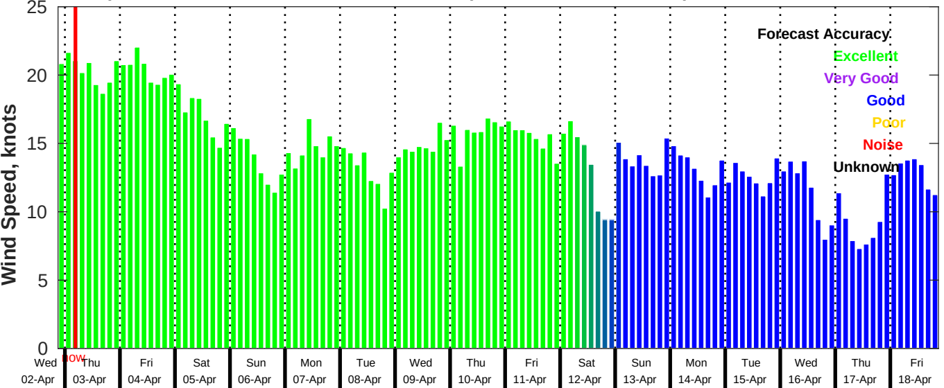
GFS Wind Speed Forecast for NDBC 41040 from 02-Apr-2025 21:00:00 to 18-Apr-2025 21:00:00
