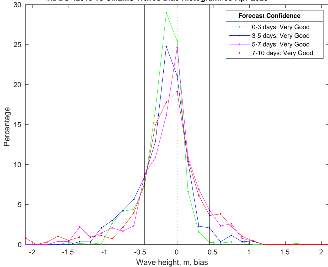
NDBC 42019 vs CMEMS Waves Bias Histogram: 03-Apr-2025
