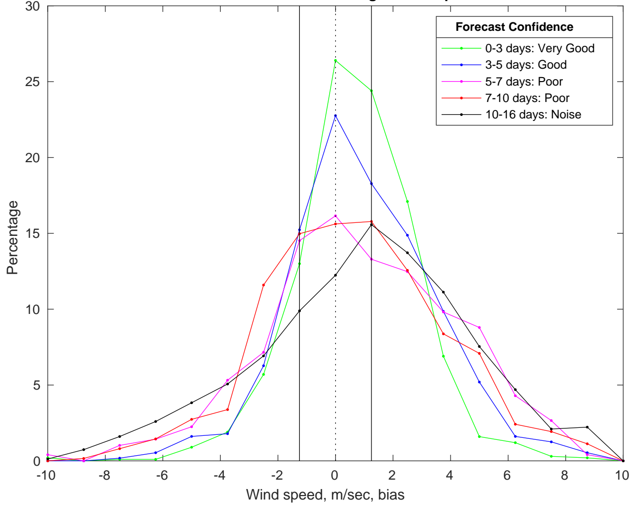
NDBC 42019 vs GFS Winds Bias Histogram: 03-Apr-2025
