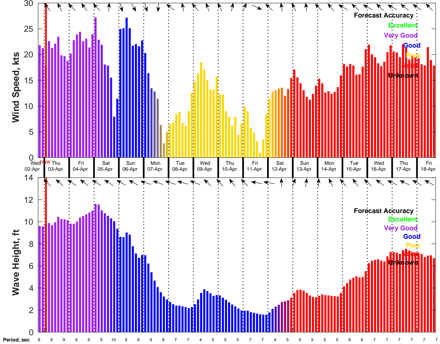
Wind & Wave Forecast for NDBC 42019 from 02-Apr-2025 18:00:00 to 18-Apr-2025 18:00:00
