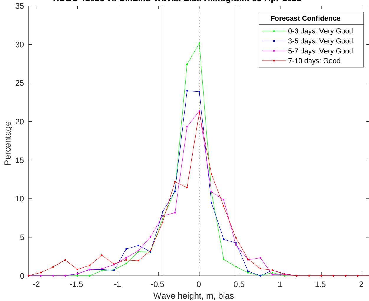
NDBC 42020 vs CMEMS Waves Bias Histogram: 03-Apr-2025
