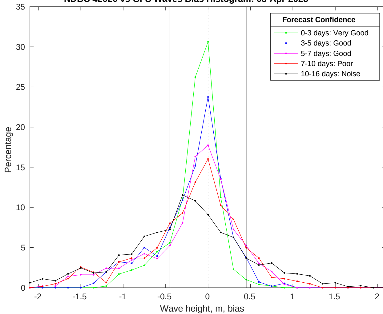
NDBC 42020 vs GFS Waves Bias Histogram: 03-Apr-2025
