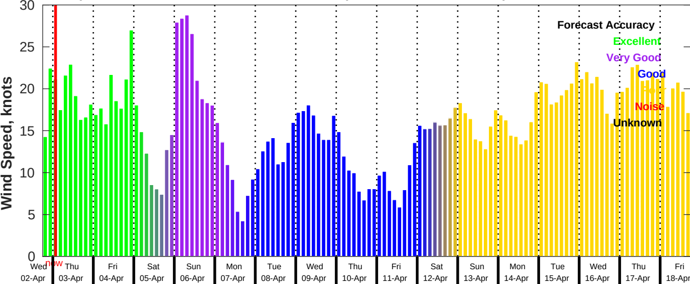
GFS Wind Speed Forecast for NDBC 42020 from 02-Apr-2025 18:00:00 to 18-Apr-2025 18:00:00
