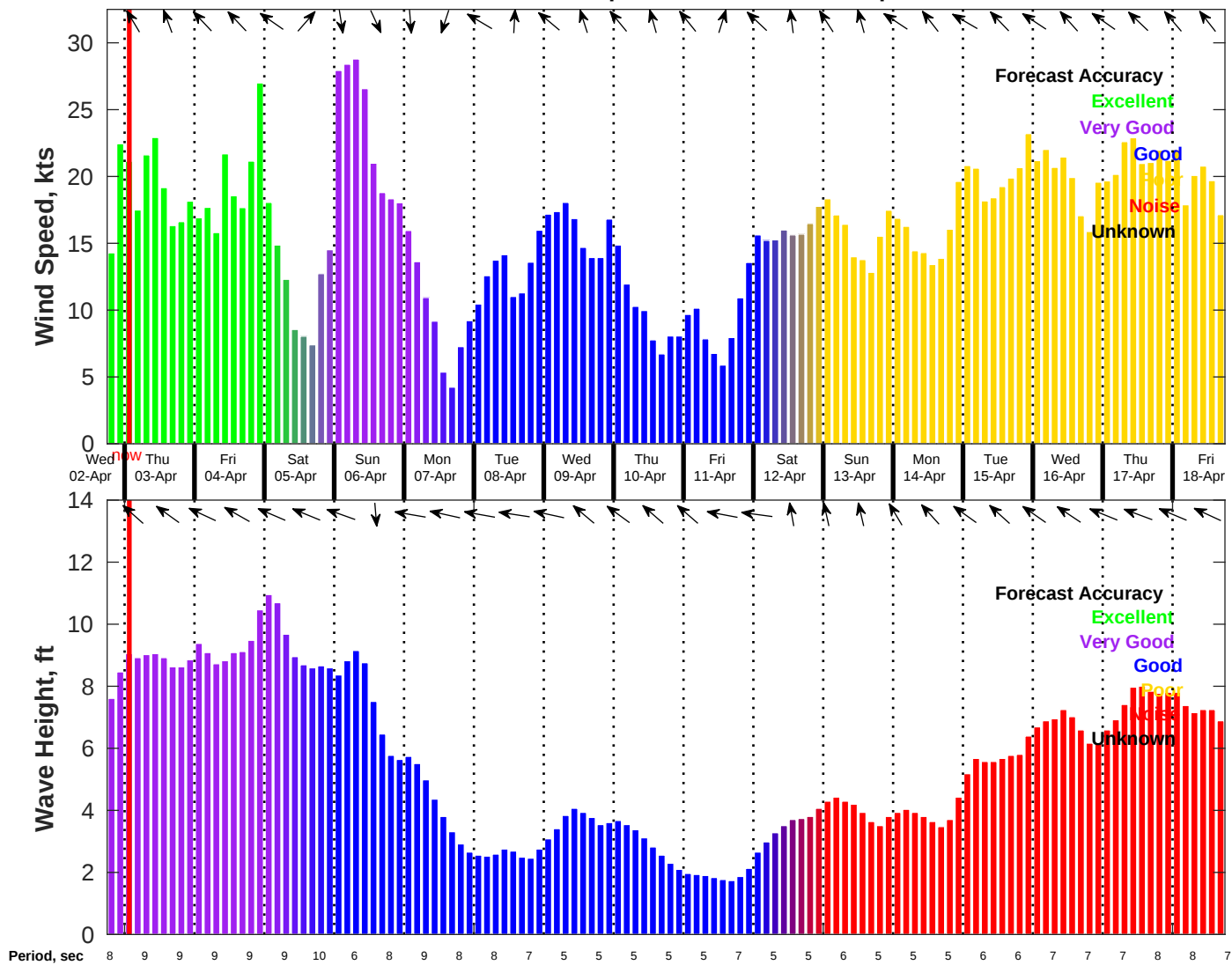
Wind & Wave Forecast for NDBC 42020 from 02-Apr-2025 18:00:00 to 18-Apr-2025 18:00:00
