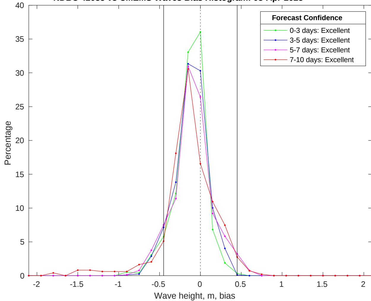
NDBC 42035 vs CMEMS Waves Bias Histogram: 03-Apr-2025
