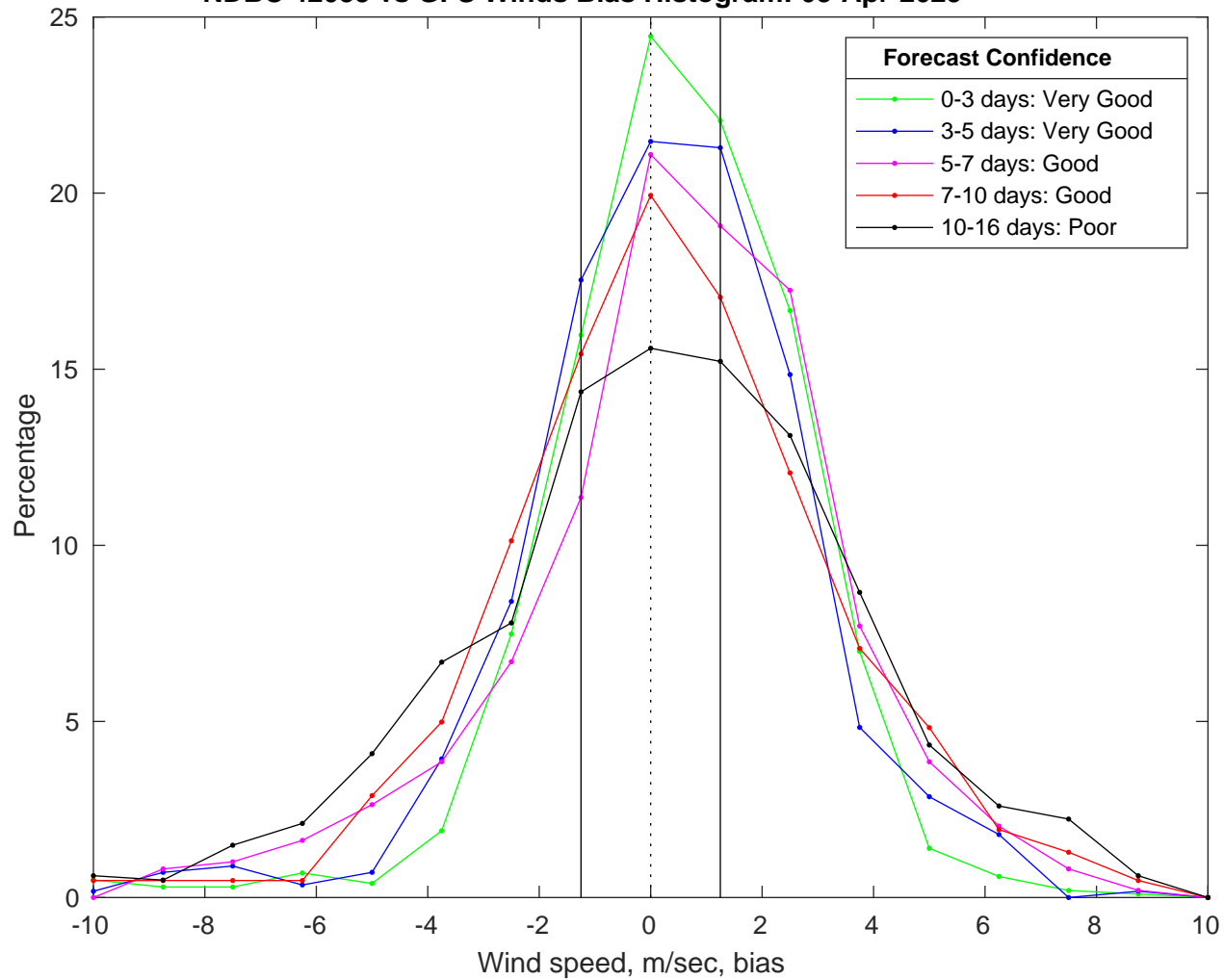
NDBC 42035 vs GFS Winds Bias Histogram: 03-Apr-2025
