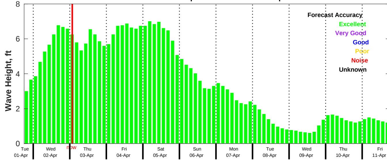
CMEMS Wave Forecast for NDBC 42035 from 01-Apr-2025 18:00:00 to 11-Apr-2025 18:00:00
