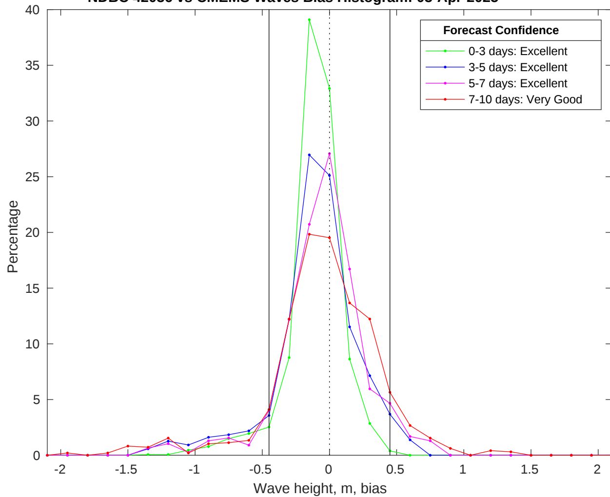
NDBC 42036 vs CMEMS Waves Bias Histogram: 03-Apr-2025
