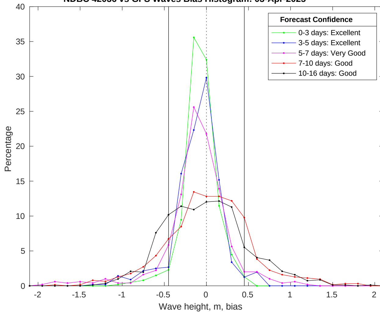
NDBC 42036 vs GFS Waves Bias Histogram: 03-Apr-2025
