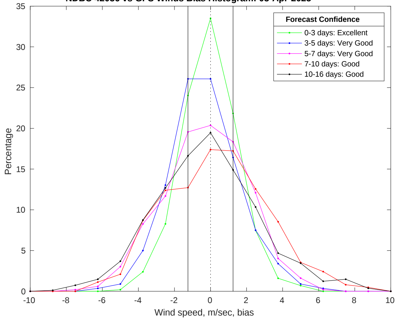
NDBC 42036 vs GFS Winds Bias Histogram: 03-Apr-2025
