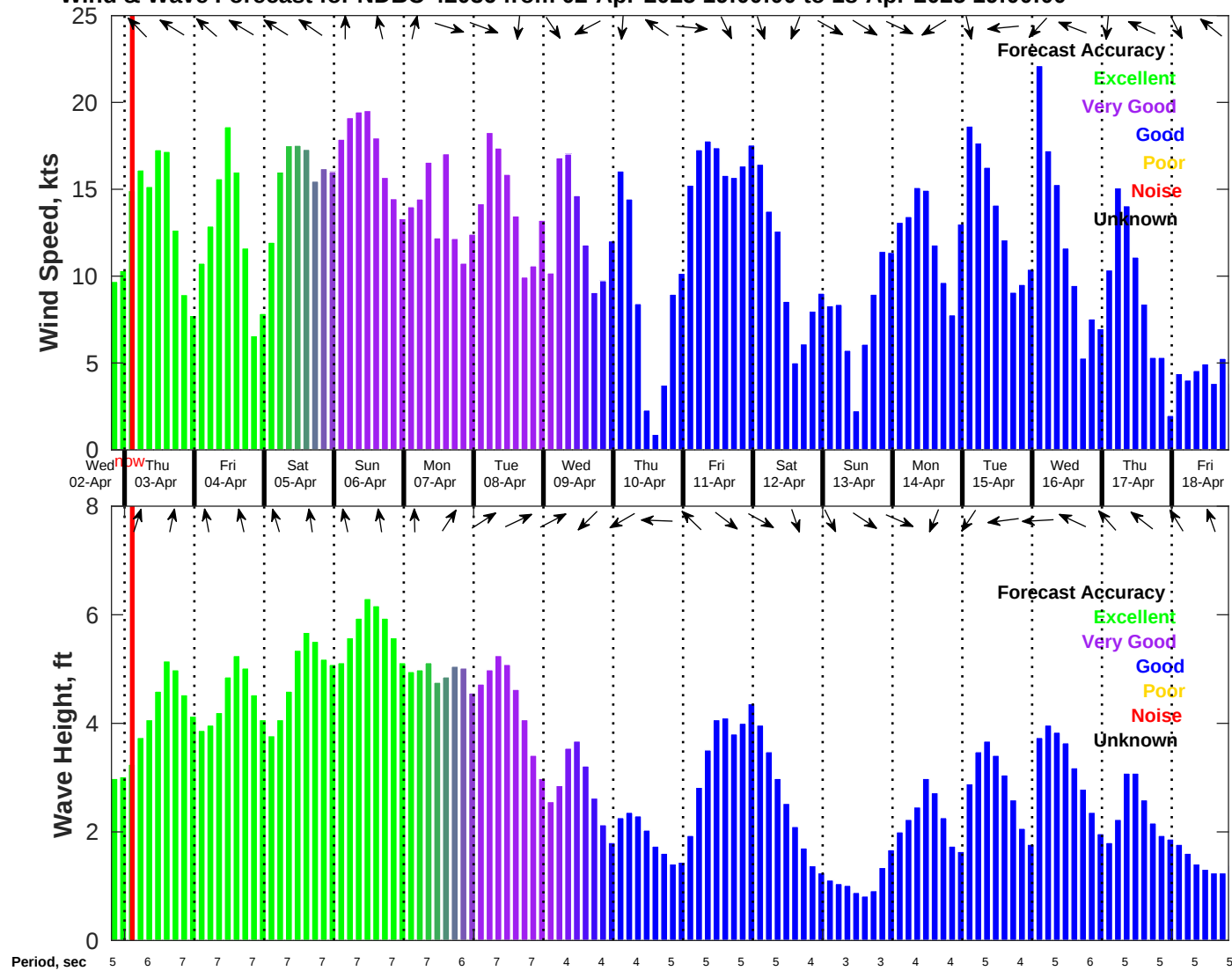
Wind & Wave Forecast for NDBC 42036 from 02-Apr-2025 19:00:00 to 18-Apr-2025 19:00:00
