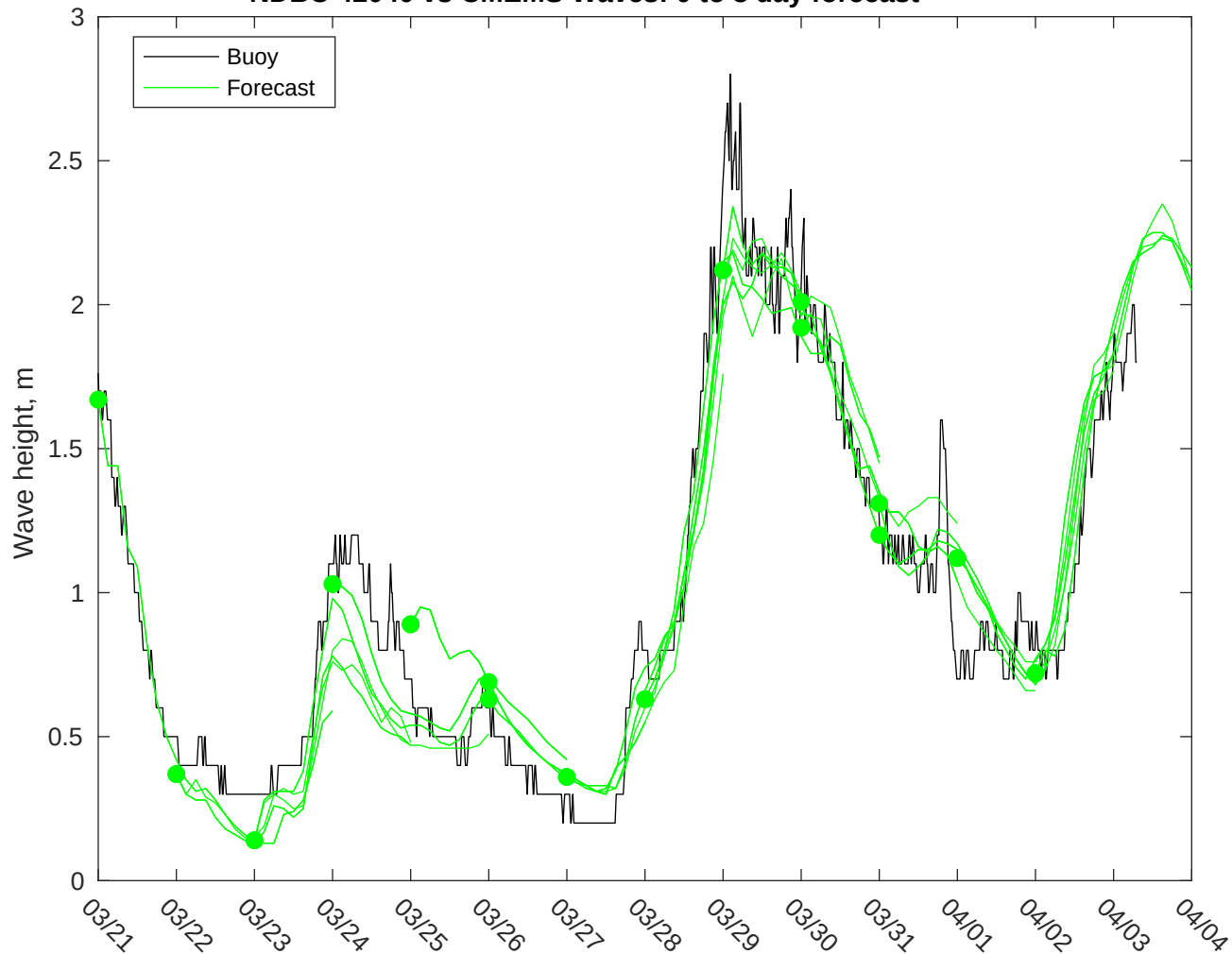
NDBC 42040 vs CMEMS Waves: 0 to 3 day forecast
