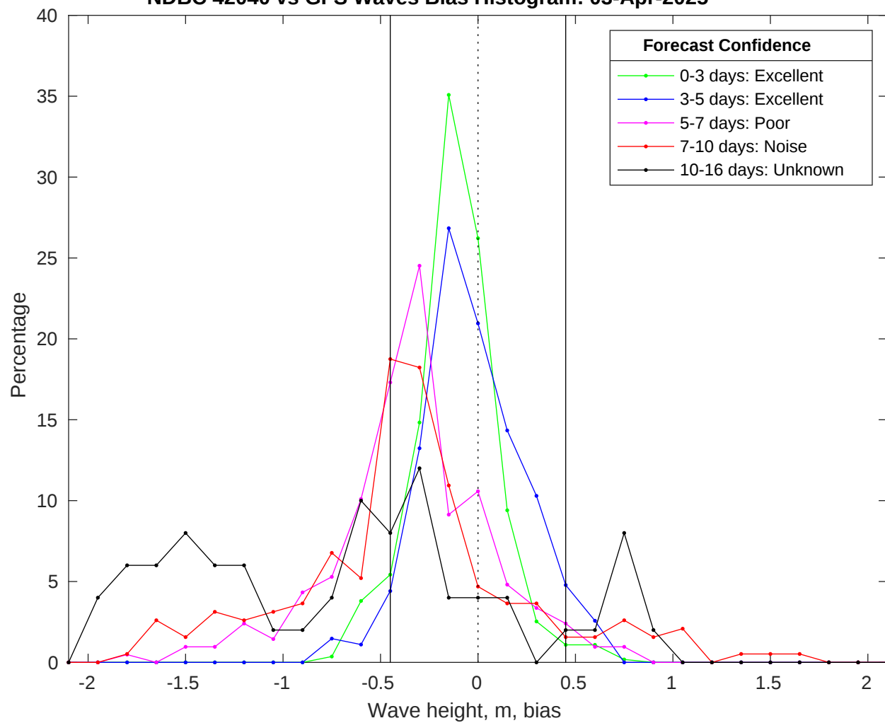
NDBC 42040 vs GFS Waves Bias Histogram: 03-Apr-2025
