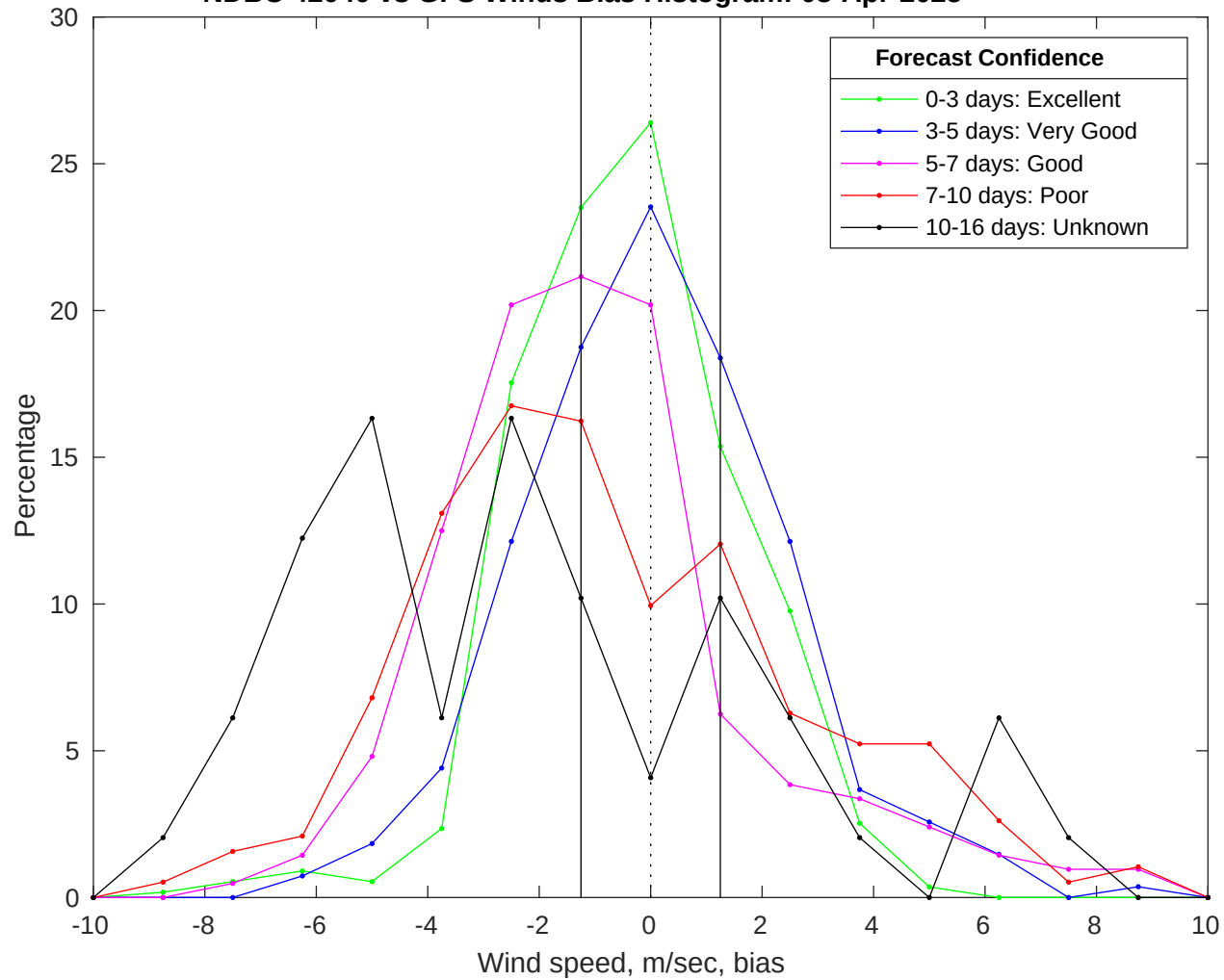
NDBC 42040 vs GFS Winds Bias Histogram: 03-Apr-2025
