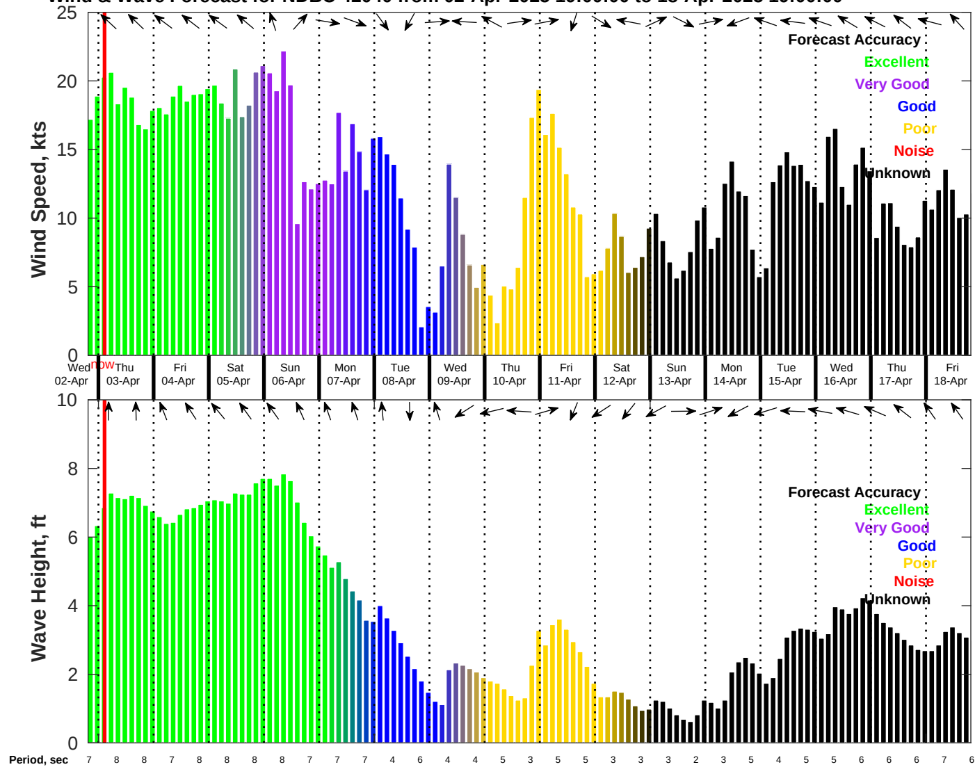
Wind & Wave Forecast for NDBC 42040 from 02-Apr-2025 19:00:00 to 18-Apr-2025 19:00:00
