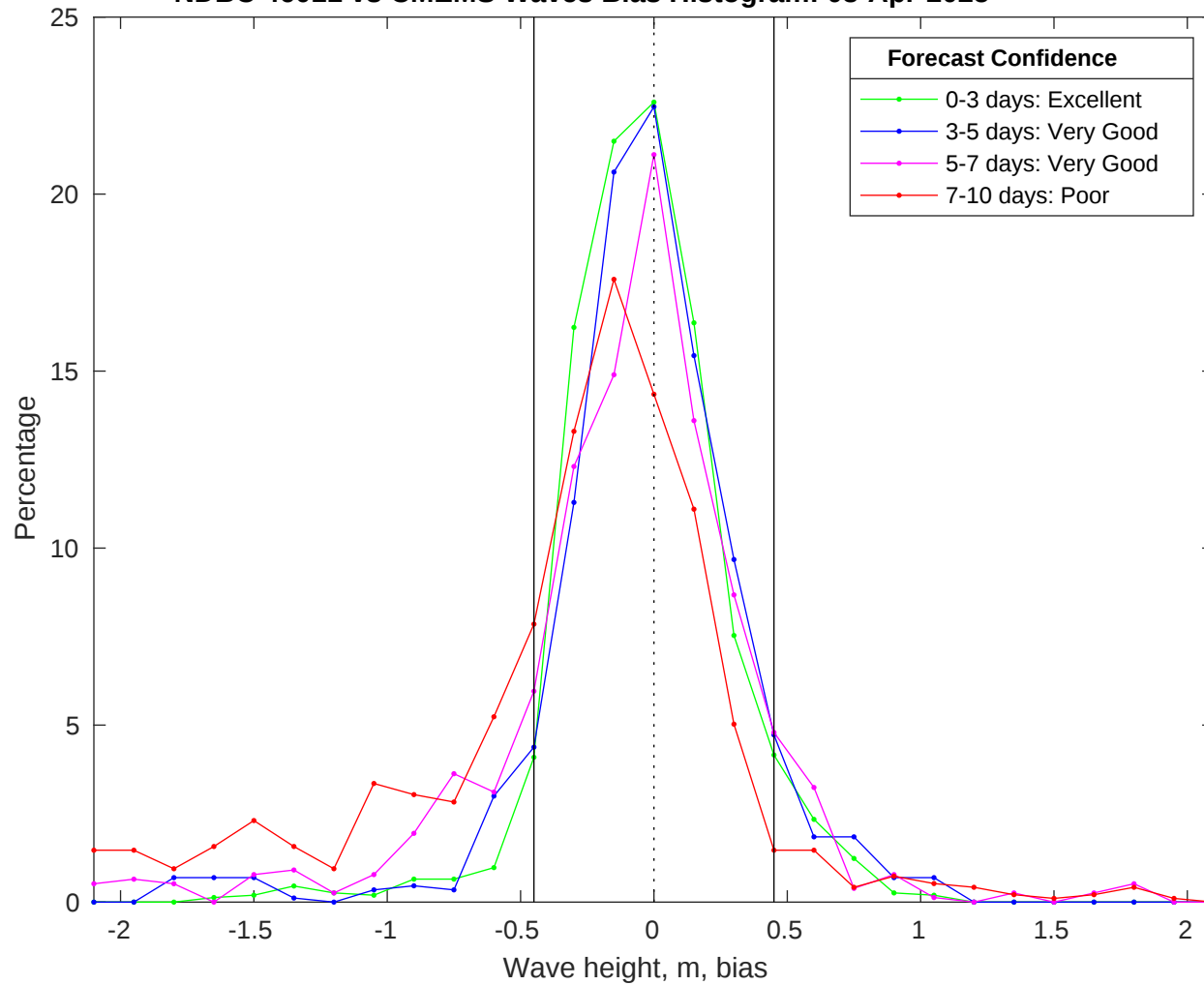
NDBC 46011 vs CMEMS Waves Bias Histogram: 03-Apr-2025
