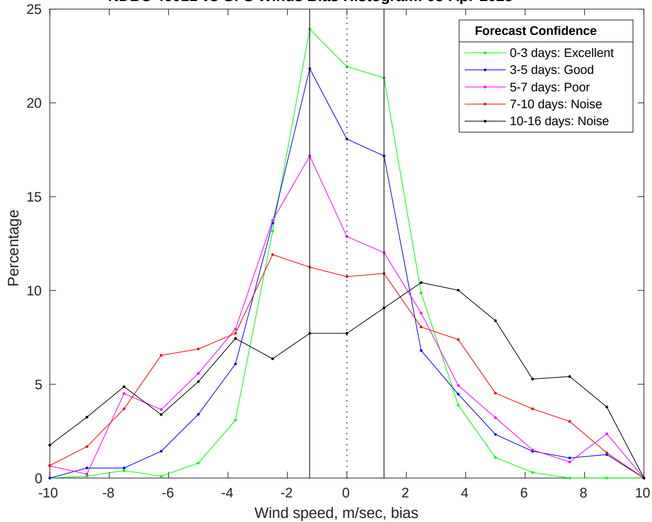
NDBC 46011 vs GFS Winds Bias Histogram: 03-Apr-2025
