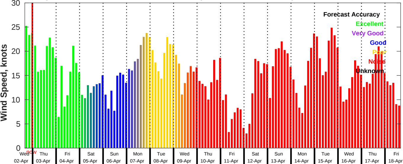
GFS Wind Speed Forecast for NDBC 46011 from 02-Apr-2025 16:00:00 to 18-Apr-2025 16:00:00
