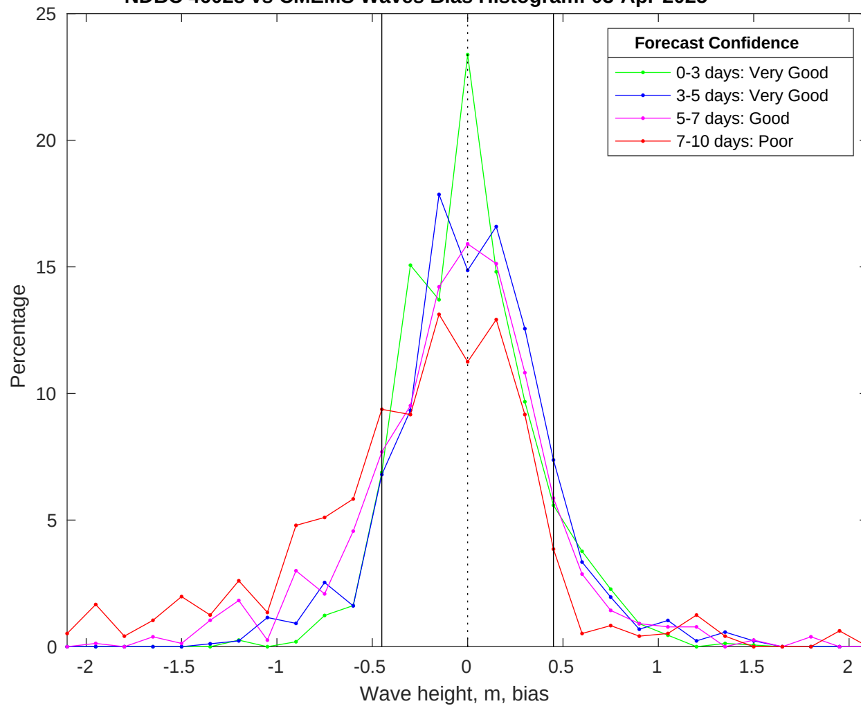
NDBC 46028 vs CMEMS Waves Bias Histogram: 03-Apr-2025
