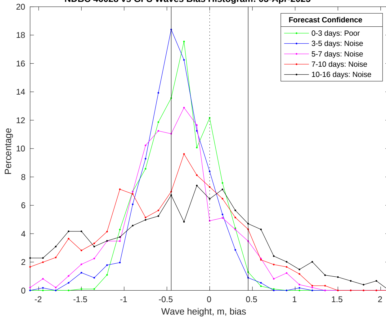
NDBC 46028 vs GFS Waves Bias Histogram: 03-Apr-2025
