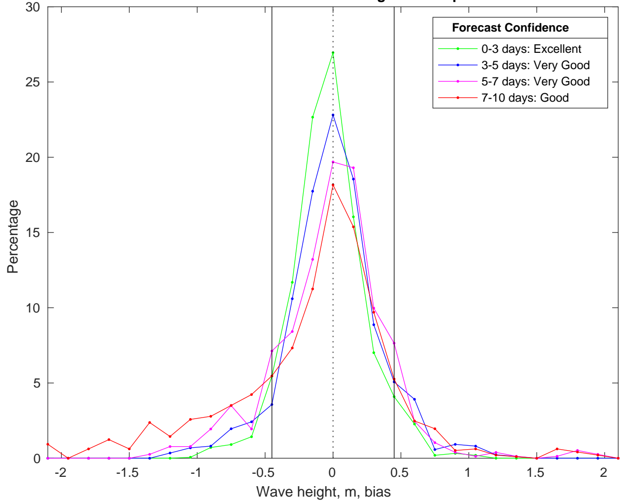
NDBC 46054 vs CMEMS Waves Bias Histogram: 03-Apr-2025
