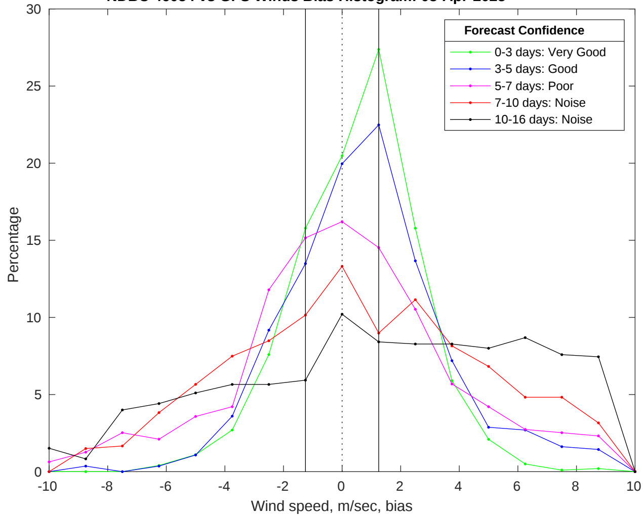
NDBC 46054 vs GFS Winds Bias Histogram: 03-Apr-2025
