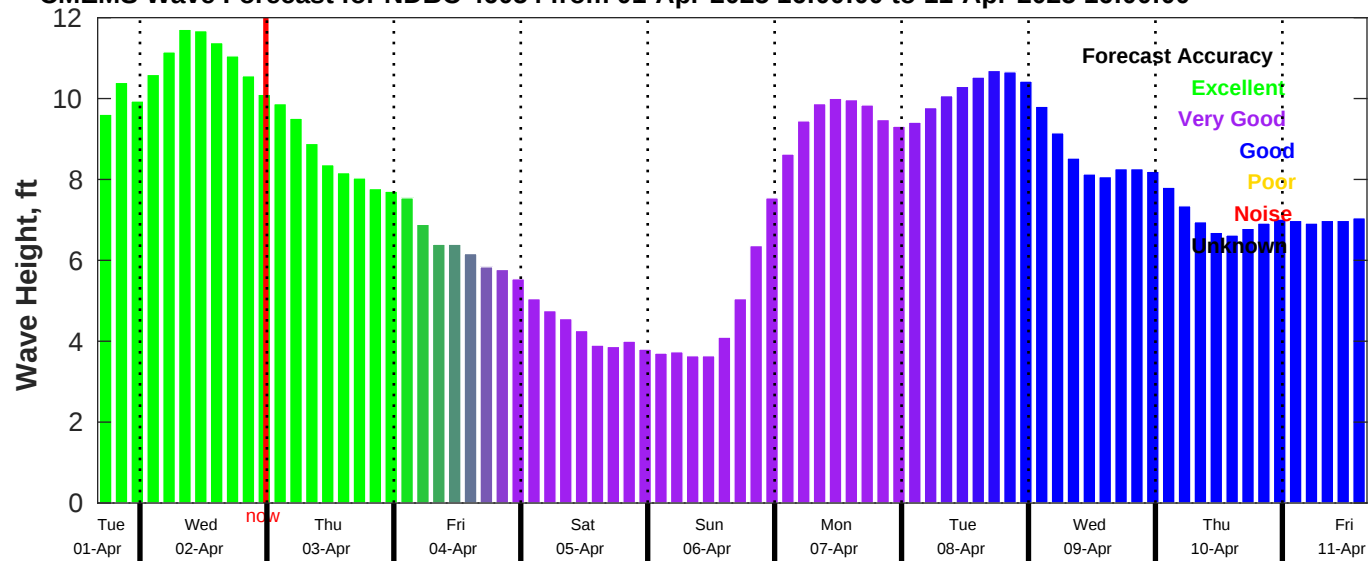
CMEMS Wave Forecast for NDBC 46054 from 01-Apr-2025 16:00:00 to 11-Apr-2025 16:00:00
