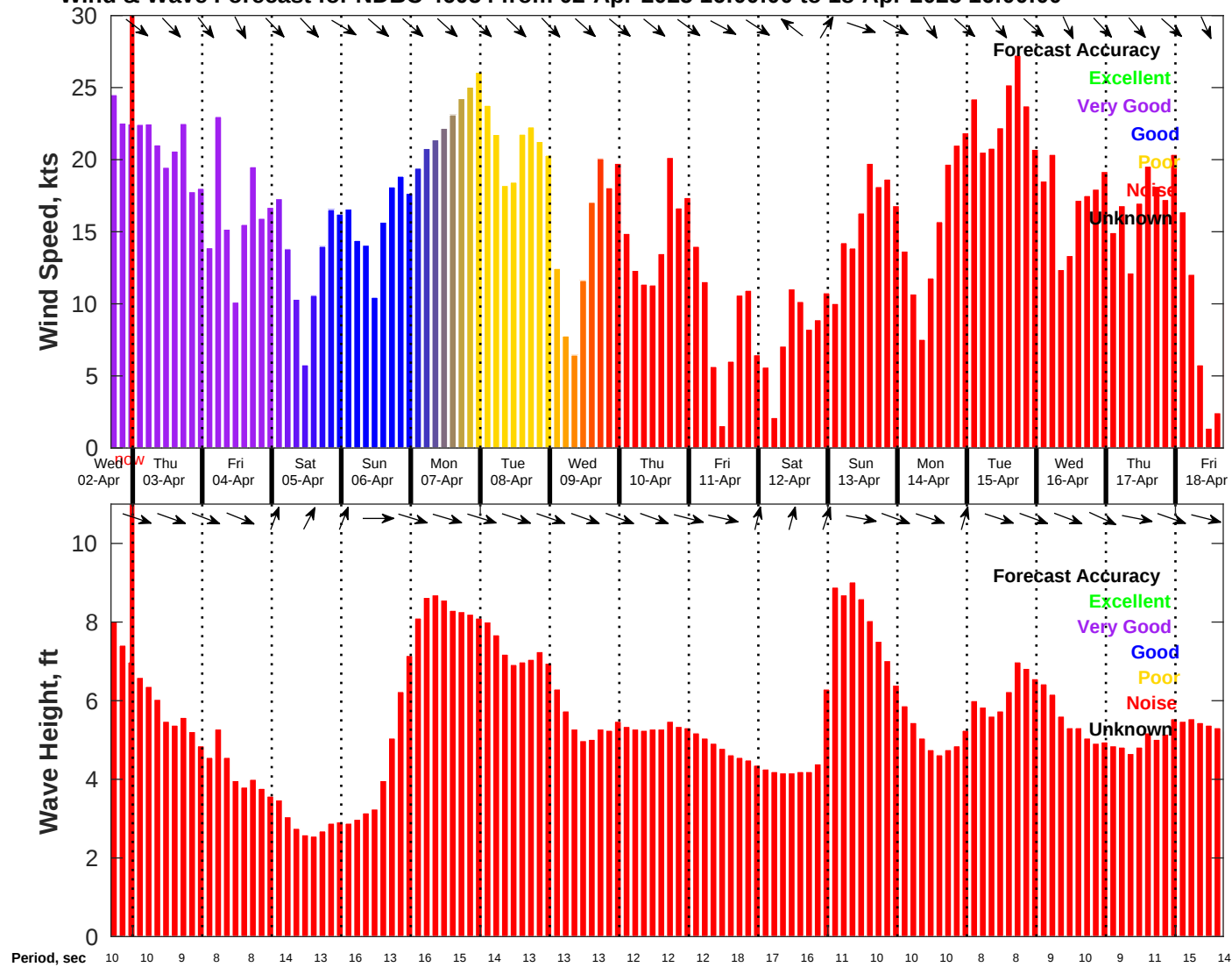
Wind & Wave Forecast for NDBC 46054 from 02-Apr-2025 16:00:00 to 18-Apr-2025 16:00:00
