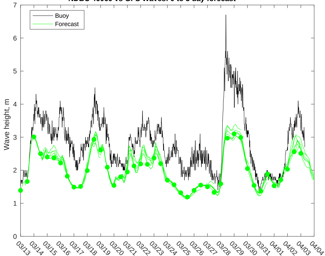
NDBC 46069 vs GFS Waves: 0 to 3 day forecast
