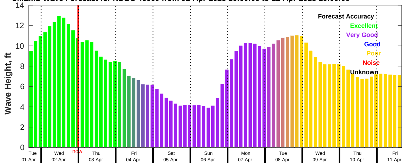
CMEMS Wave Forecast for NDBC 46069 from 01-Apr-2025 16:00:00 to 11-Apr-2025 16:00:00
